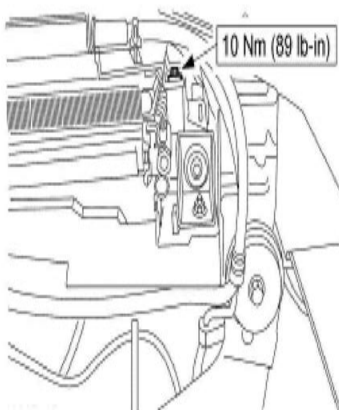
Fig. 88: Removing Condenser-To-Radiator Belts Courtesy of FORD MOTOR CO.
